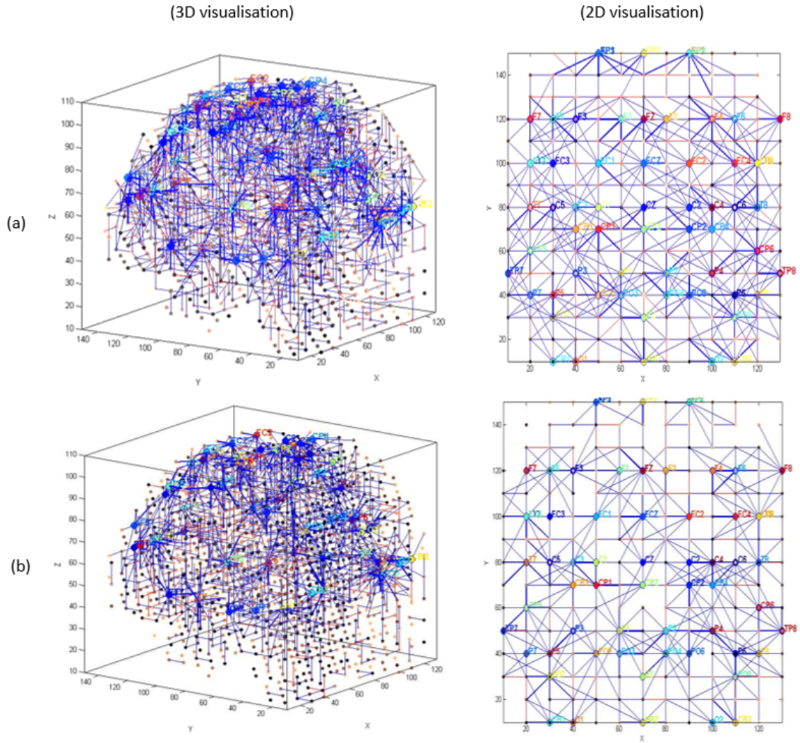
Figure 7. The neuronal connections created for the experimental group in the brain-inspired SNN models reflect the functional connectivity in response to distractor stimuli (a) before (T1) and (b) after the mindfulness training (T2).
